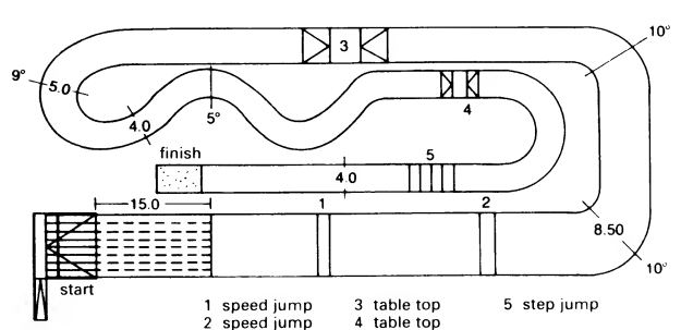
⑭ BMX track at the IFMA '84 in Cologne
